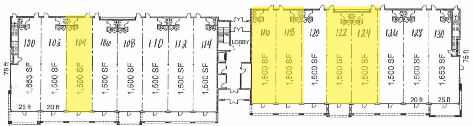
FIRST FLOOR RETAIL FLOOR PLAN
